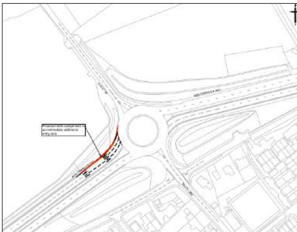
Figure 4-2: Proposed Layout – A228 Peninsula Way / Main Road Hoo
