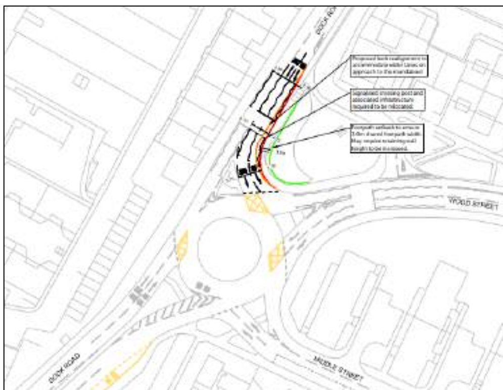
Figure 11-2: Proposed Layout – Dock Road / Middle Street / Wood Street
