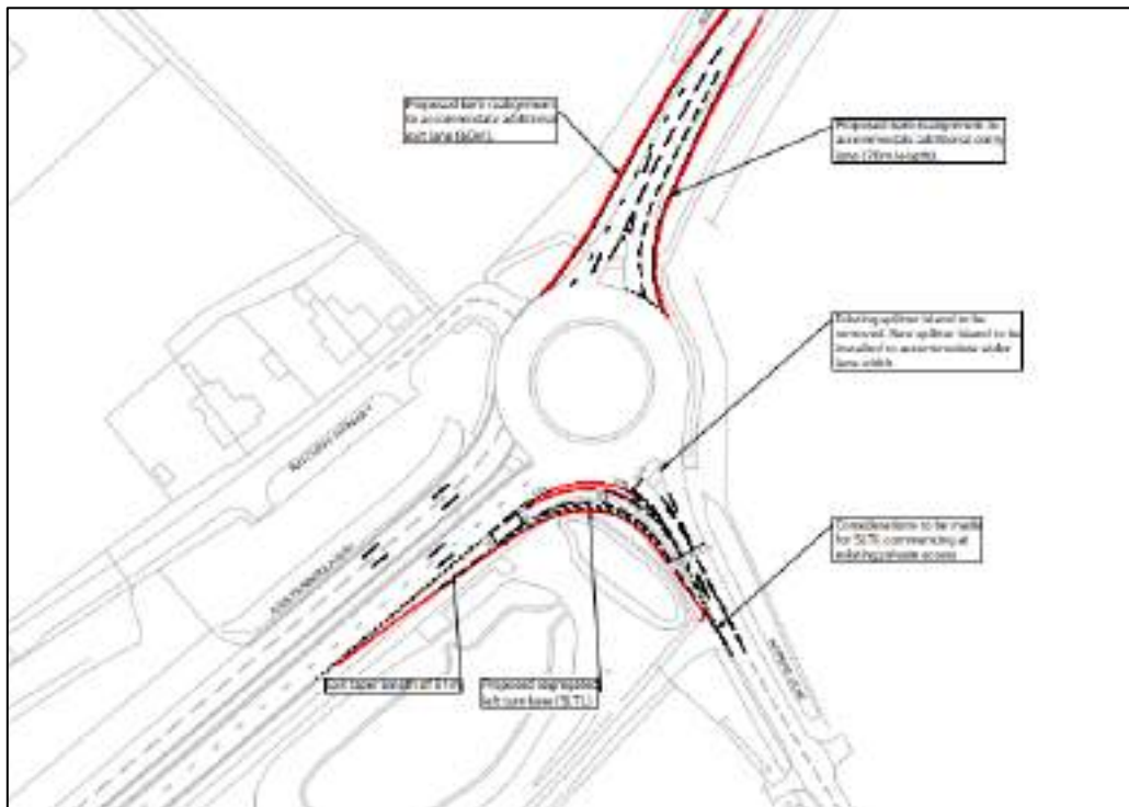
Figure 5-2: Proposed Layout – A228 Peninsula Way / Main Road Hoo – Option 1
