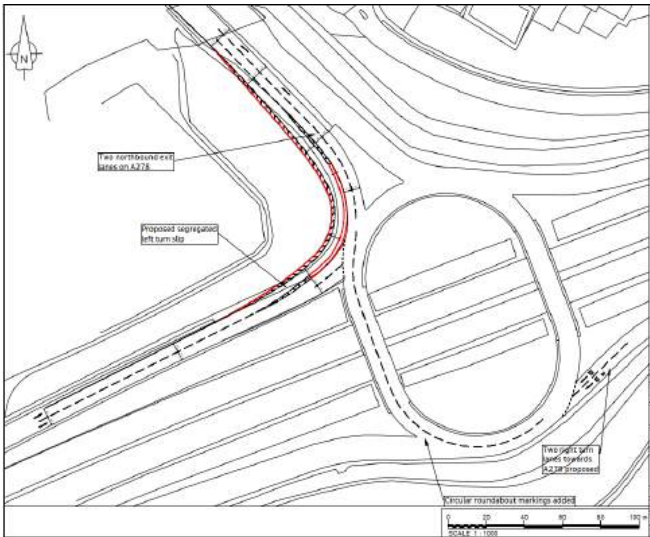
Figure 13-3: Proposed Interim Layout – M2J4
