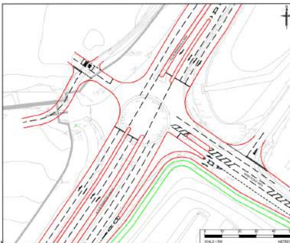
Figure 3-2: Proposed Layout – A228 Peninsula Way / Main Road Hoo
