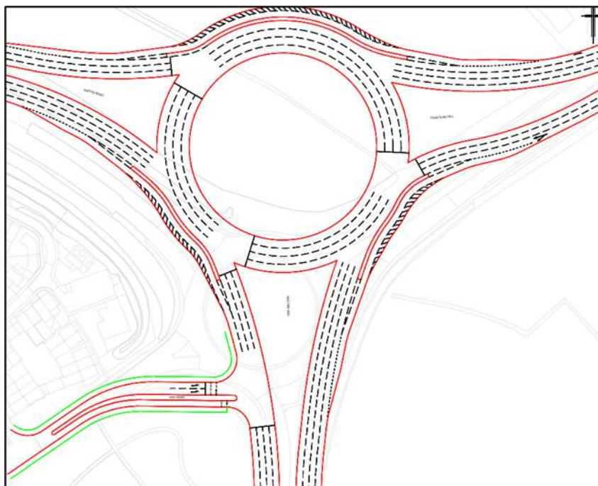
Figure 2-2: Proposed Layout – Four Elms
