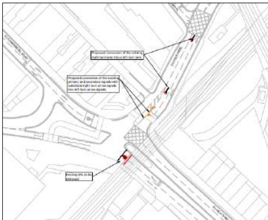
Figure 7-2: Proposed Layout – A2 High Street /Station Road
